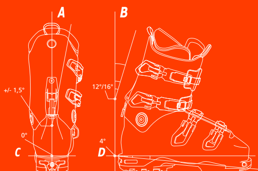
A. cuff cant +/- 1,5° B. enhanced fore-aft balance, leverage 12° without spoiler and 16° with forward lean spoiler C. enhanced edge release, speed 0° degree sole cant D. enhanced balance, steering 4° ramp angle
