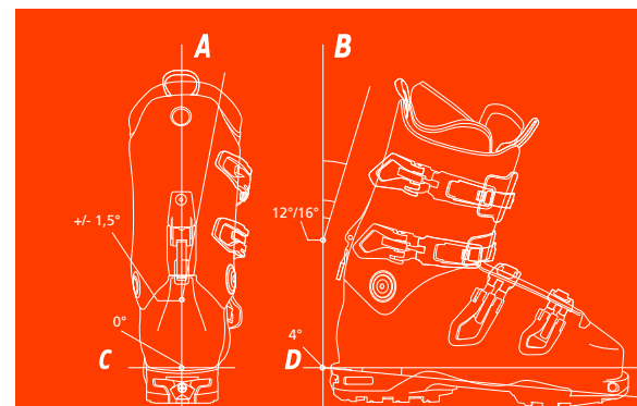
A. cuff cant +/- 1,5° B. enhanced fore-aft balance, leverage 12° without spoiler and 16° with forward lean spoiler C. enhanced edge release, speed 0° degree sole cant D. enhanced balance, steering 4° ramp angle
